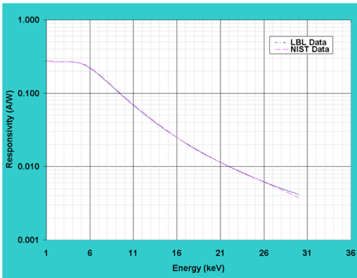
Figure 2: Responsivity calculated using both NIST and LBL transmission values for the photoelectric effect, 52 \mu\text{m} effective Si thicknesses.
