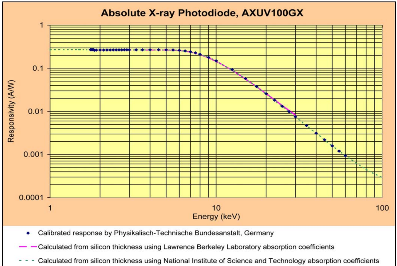
Figure 3: Responsivity of the AXUV100GX photodiode, compared against calculations using both NIST and LBL transmission values, 104 \mu\text{m} effective Si thicknesses.
