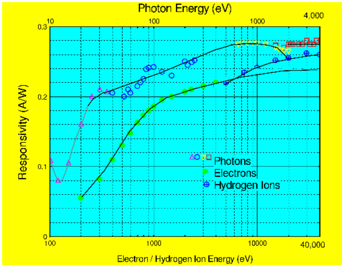
Figure 1: Photon and electron responsivity for the AXUV photodiode.
