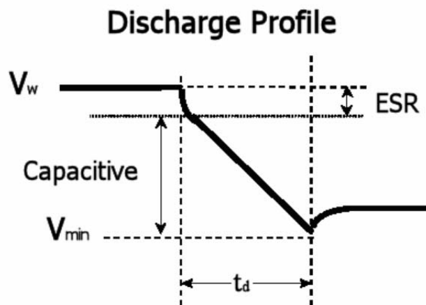
Figure 1: Constant current discharge profile
